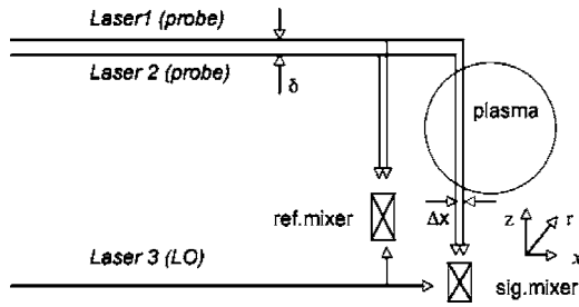
FIG. 1. Schematic of the differential interferometer experimental setup. Note that beam offsets at the source ( \delta ) and in the plasma ( \Delta x ) are different due to an optical system with out-of-plane non-45° bends that are not pictured.
