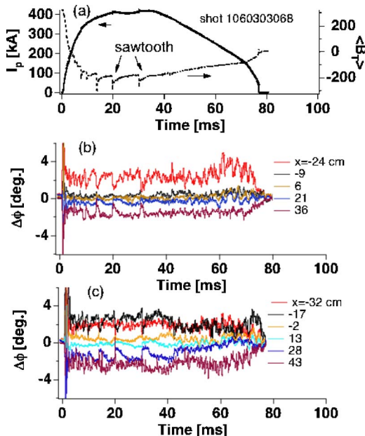
FIG. 2. (a) Time history of discharge current and average toroidal magnetic field. The arrows point to sawtooth crashes. [(b) and (c)] Time history of the differential interferometer for 11 chords where x denotes the impact parameter of the laser beams and \delta=3.5 mm.
