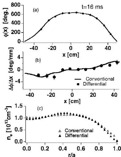
FIG. 5. (a) Measured phase profile \phi(x) at t=16 ms for conventional interferometer (solid circles); the solid line is spline fit to measured points; (b) first derivative of phase, d\phi/dx , is calculated and shown as solid line. The direct measurements from differential interferometer are shown by solid circles using \Delta x=1.20 mm; (c) density profile comparison using the conventional and differential interferometer techniques.
