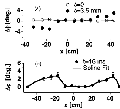
FIG. 3. (a) Phase difference profile with separations \delta=0 (open circles) and \delta\sim 3.5 mm (solid circles); (b) spline fit to measured |\Delta\phi| profile used for inversion.
